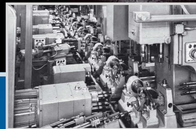
1951 – Transfer line for machining swivel bearings.
