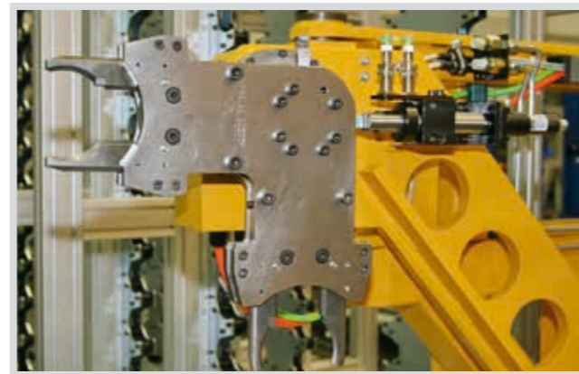
Tool gripper.
